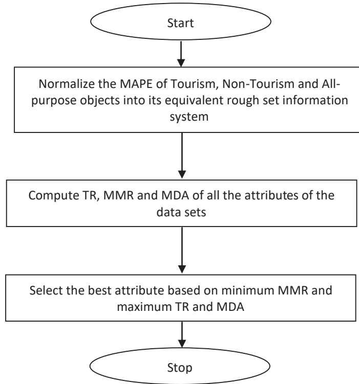
Figure 1. The Stages of Building best forecasting models.
