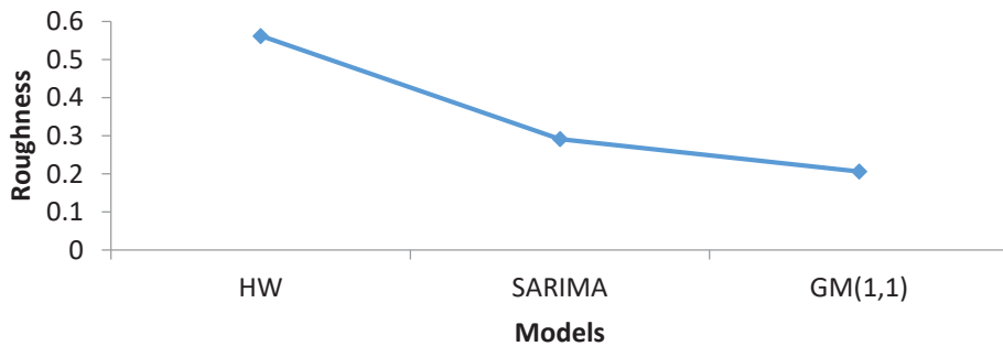
Figure 4. The roughness of HW, SARIMA and GM (1, 1) models based on TR criterion for Case 2
